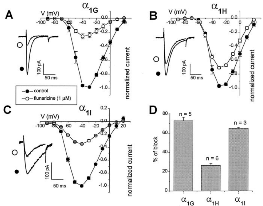
Figure 4. Differential blockade of T-type Ca channels by the diphenylpiperazine flunarizine. Mean I - V relationships of T-type currents in the absence (filled circles) or presence (open circles) of flunarizine (1 \mu M), were obtained from normalized currents (mean \pm SE from 3–6 cells) through \alpha_{1G} (A), \alpha_{1H} (B), and \alpha_{1I} (C). Normalized mean I - V data represent the mean \pm SE from three to six cells. Insets show representative current traces in absence (control, filled circles) and presence (open circles) of 1 \mu M flunarizine, elicited with test pulses to -40 mV ( \alpha_{1G} , \alpha_{1I} ) or -30 mV ( \alpha_{1H} ). D, Flunarizine (1 \mu M) differentially inhibited the cloned T-type currents, inhibiting \alpha_{1G} and \alpha_{1I} more potently ( \sim 70\% ) than \alpha_{1H} ( \sim 30\% ).
