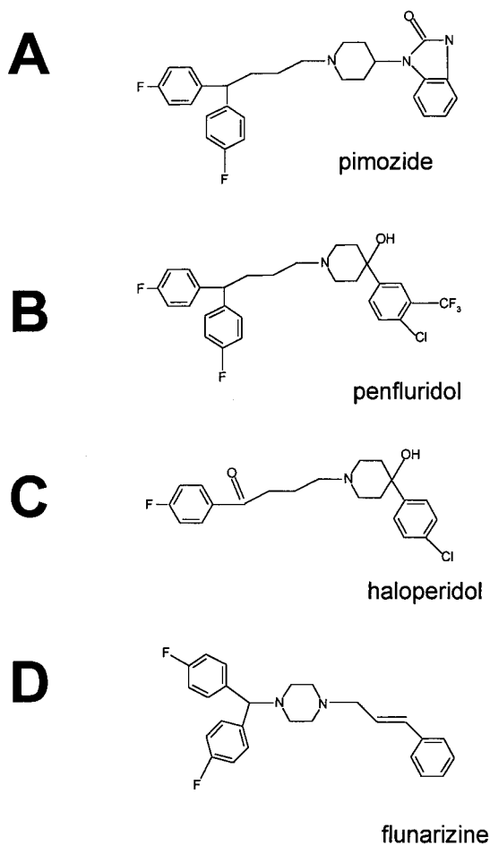
Figure 1. Chemical structures of the three different structural classes of neuroleptic agents used in this study: the DPBPs pimozide (A) and penfluridol (B). An example of a butyrophenone (C, haloperidol) and a diphenylpiperazine, flunarizine (D).
